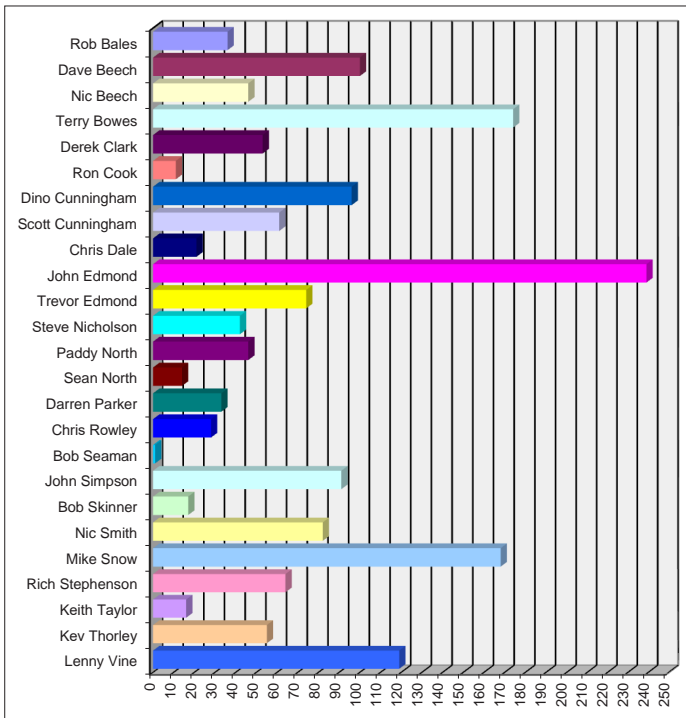
Individual Weights
