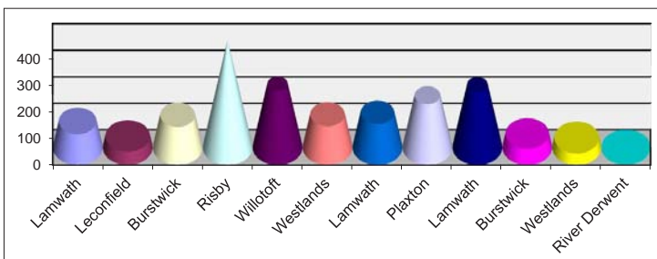
Venue Weights
